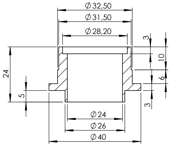
Bushing Cod. 204640
