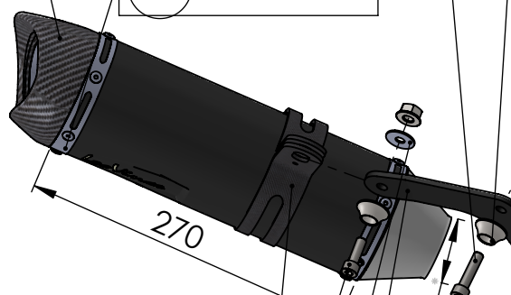
Carbon bracket FM4S Cod.307572505
