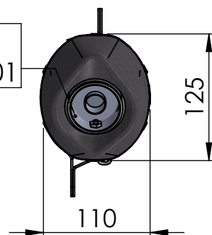
Welded s.s. flange "43E" cod.206308
