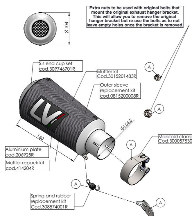
ART. 15203C SPARE PARTS YAMAHA MT-10/SP Ⓐ FITTING KIT cod.3015203601R
