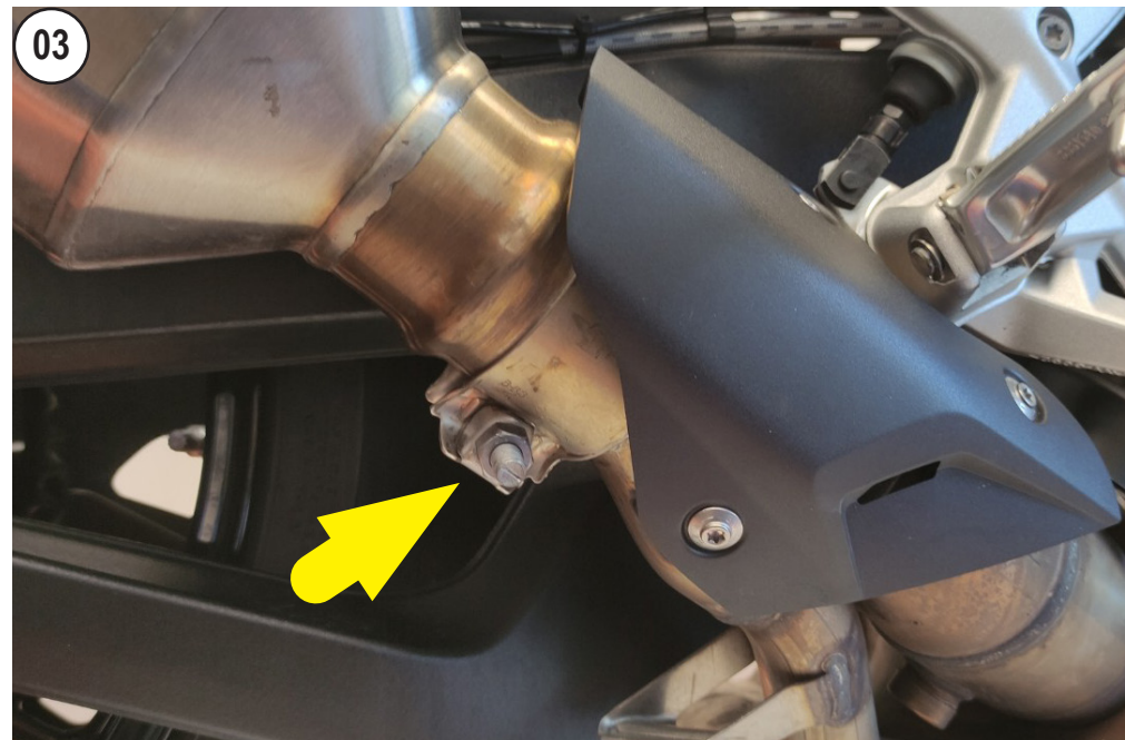
LOOSE THE CLAMP
