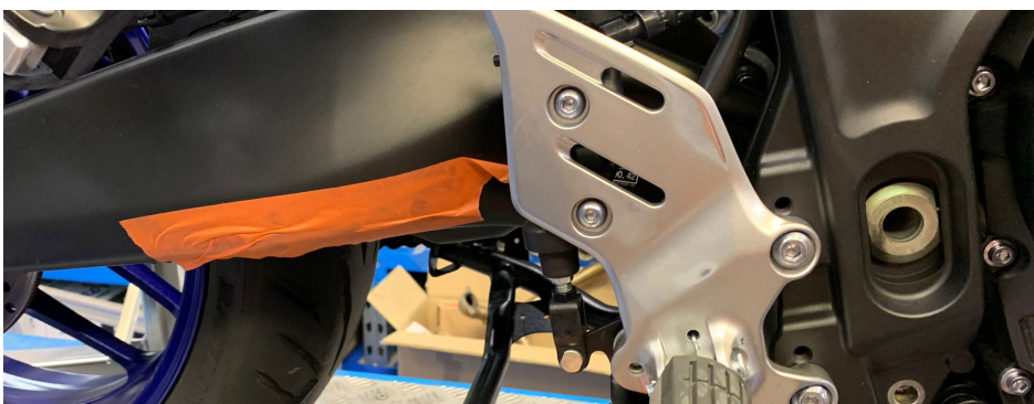
PHOTO 12 - Install the Muffler and Remove the tape
