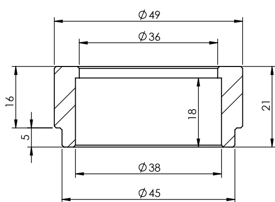
S.S. Bushing kit P/N 207351R
