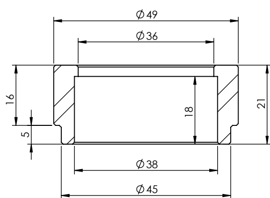
S.S. Bushing P/N 207351
