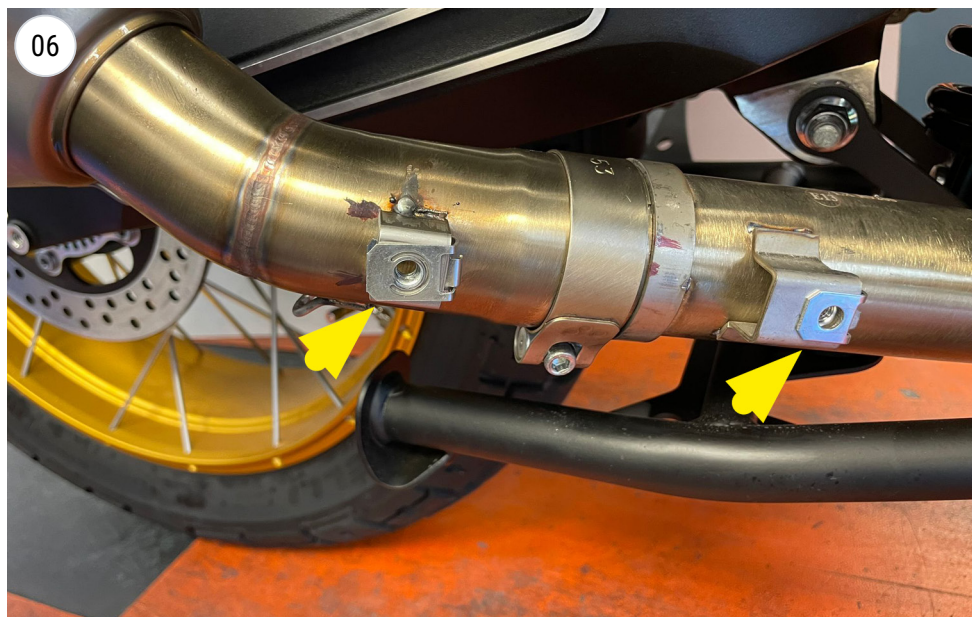
fit the mounting plate
