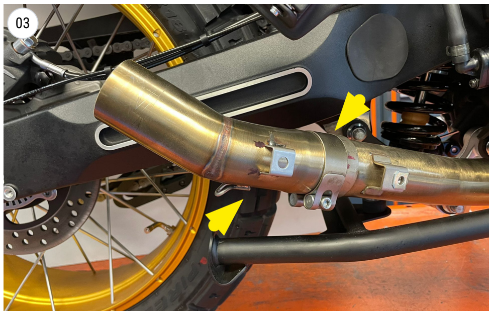
fit the pipe with the clamp
